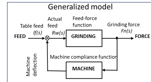
Block diagram of grinding
