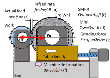
Grinding system
