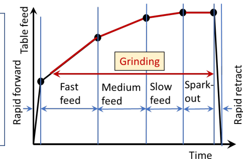
Grinding cycle design
